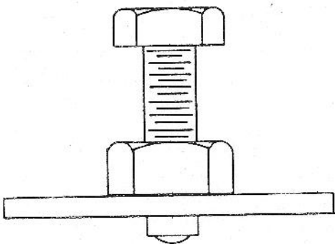
110 FLYWHEEL PULLER
