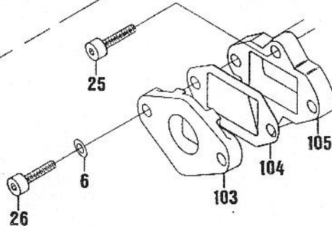
32 MM ADAPTER
